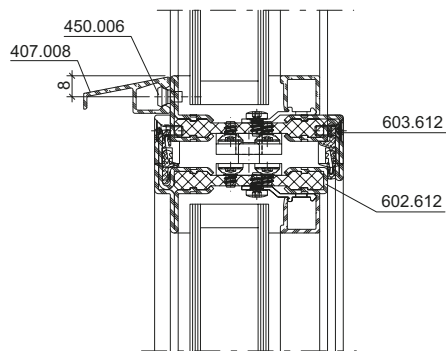
Installation weatherbar 407.008/407.009 (Inward-opening sash)
